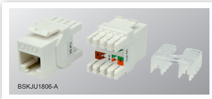
Infrastone Cat6A unshielded keystone jacks (180 degree)
