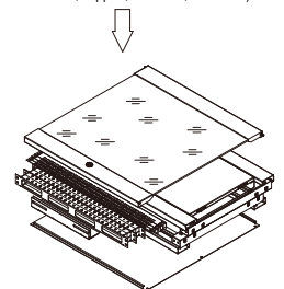
B package(back door, L guide rail, frame, mounting plate, frame holder, support, side door, front door)
